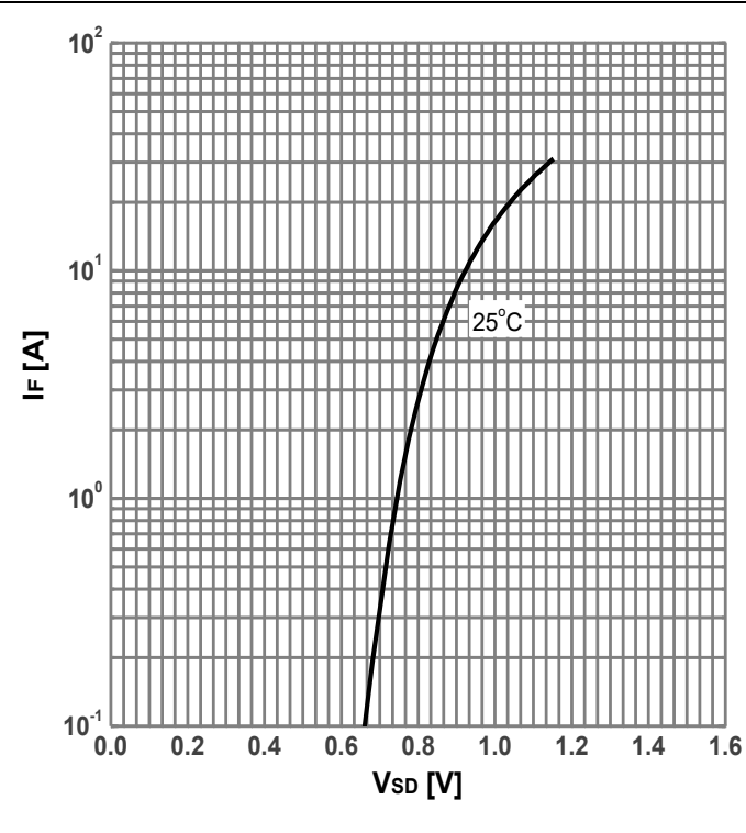
Diagram 10: Forward characteristics of reverse diode
