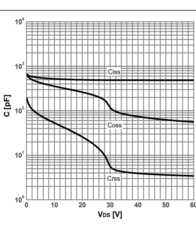
Diagram 12: Typ. capacitances
