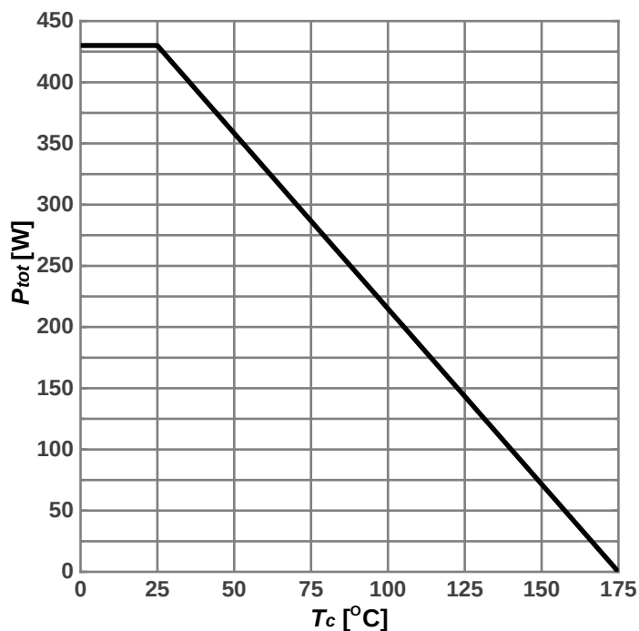
Diagram 1: Power dissipation
