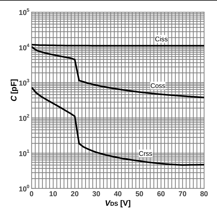
Diagram 12: Typ. capacitances
