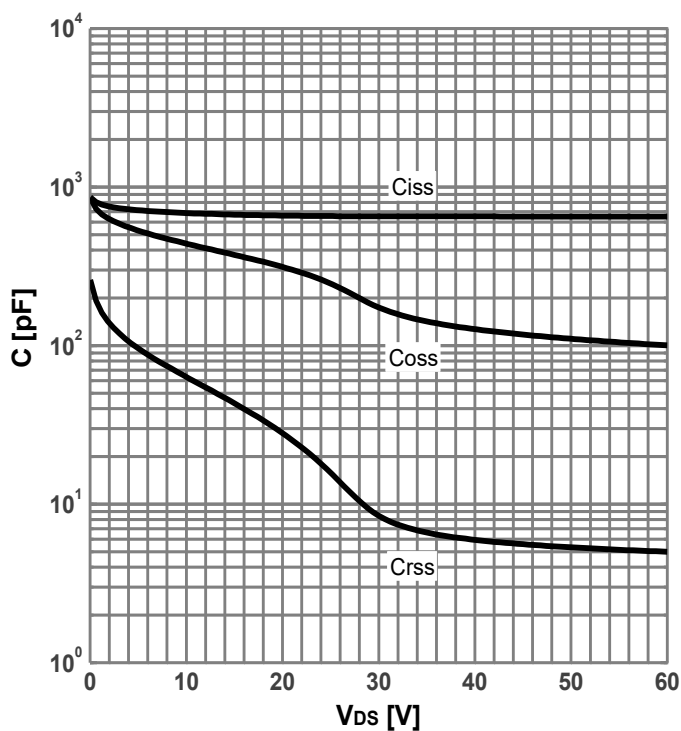
Diagram 12: Typ. capacitances
