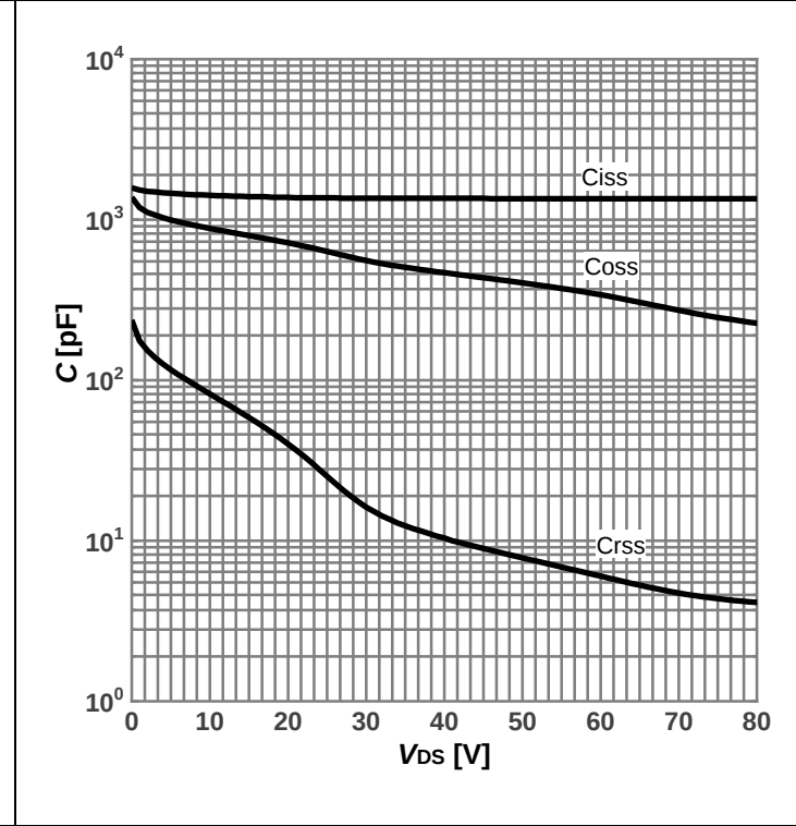
Diagram 12: Typ. capacitances
