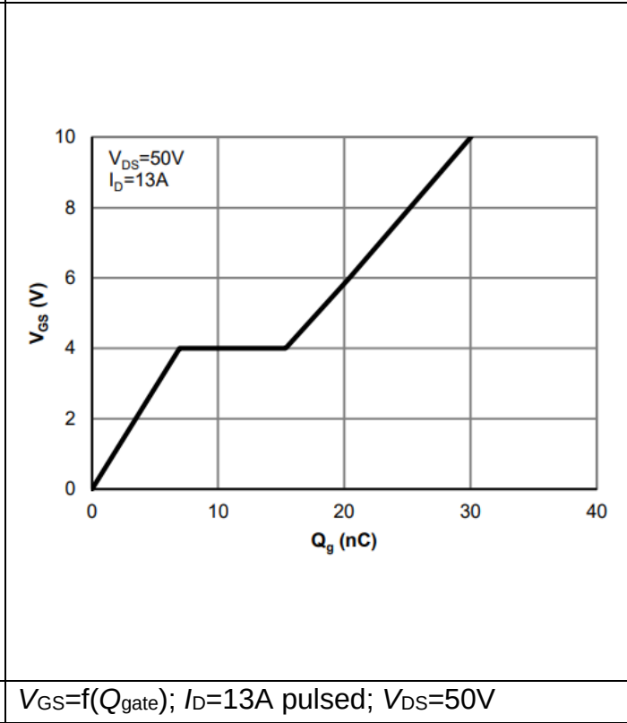
Diagram 13 Typ. gate charge
