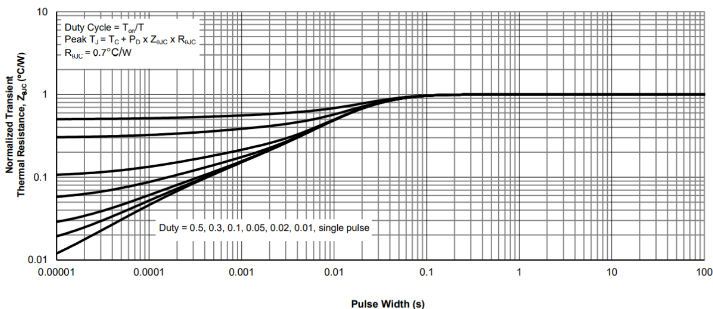
Diagram 3: Normalized Maximum Transient Thermal Impedance
