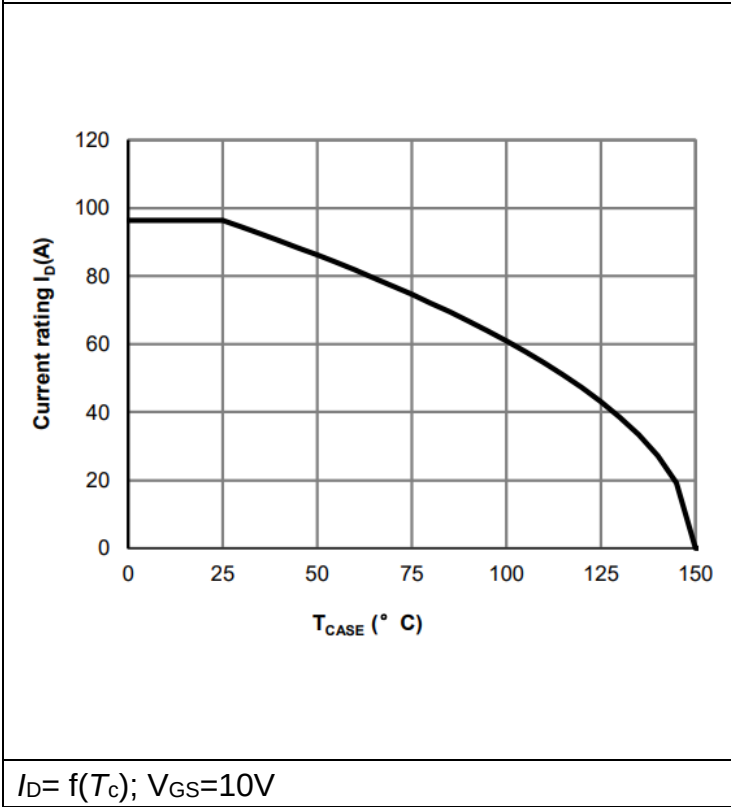
Diagram 12: Maximum Drain Current
