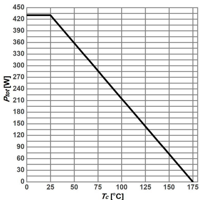
Diagram 1: Power dissipation
