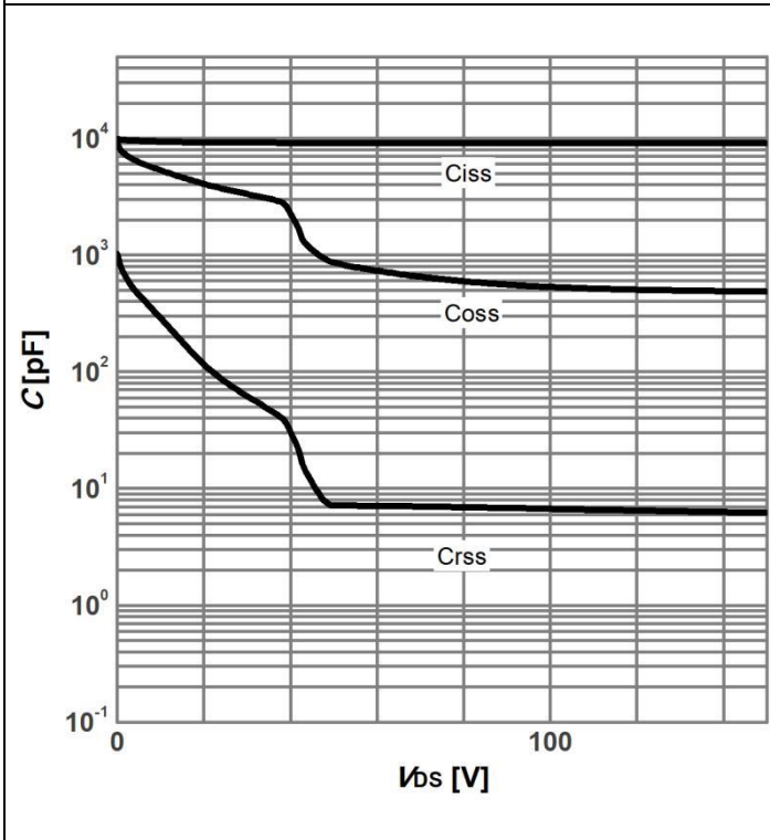
Diagram 13: Typ. capacitances
