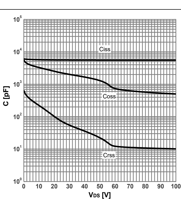
Diagram 12: Typ. capacitances
