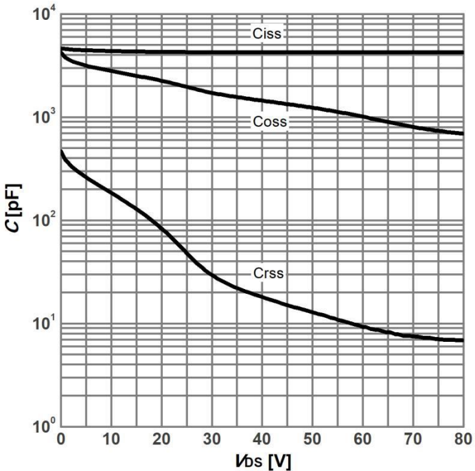
Diagram 12: Typ. capacitances
