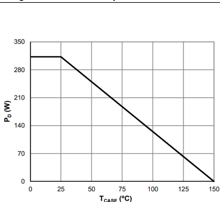
Diagram 1: Power dissipation
