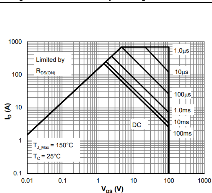
Diagram 2: Max. Safe operating area
