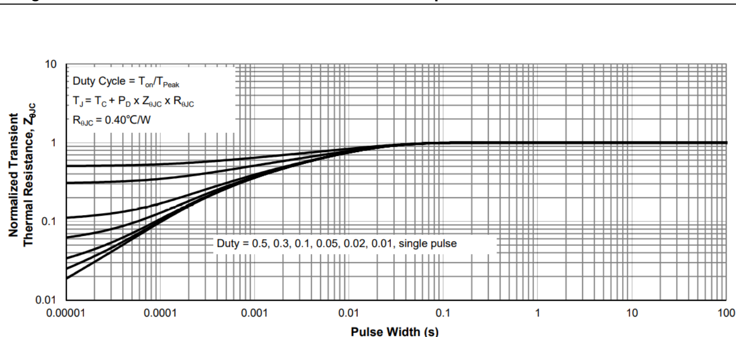
Diagram 3: Normalized Maximum Transient Thermal Impedance
