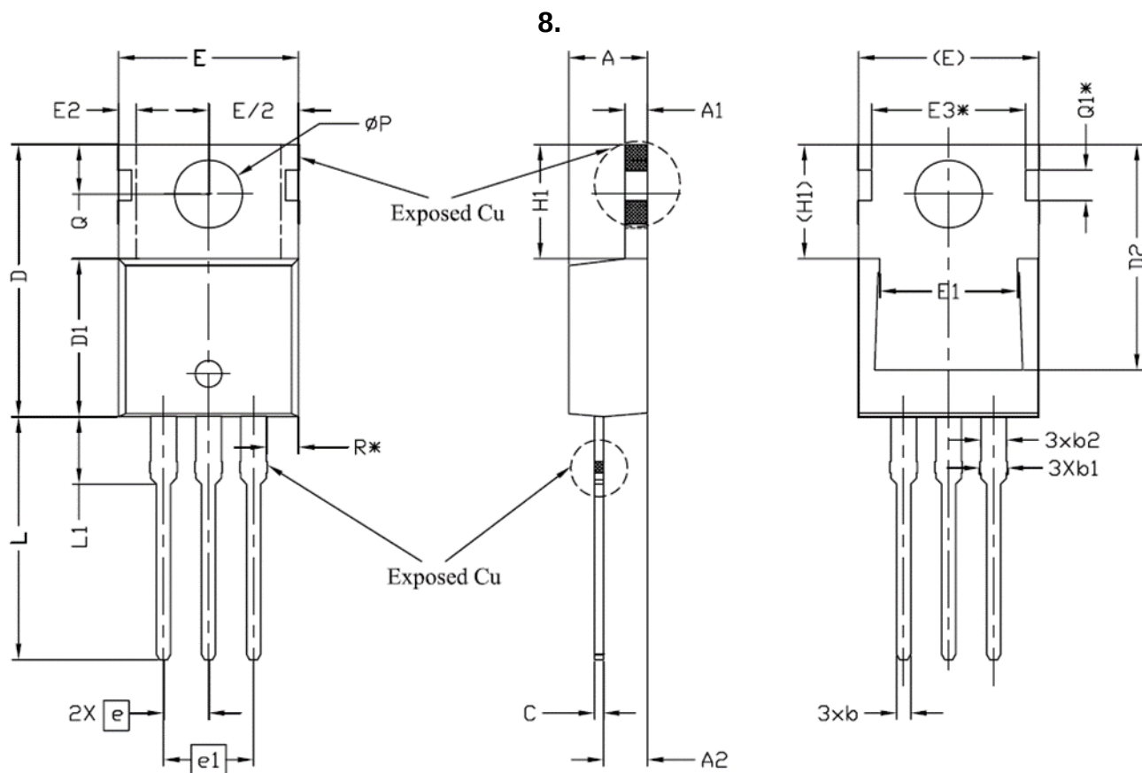
Figure 1 Outline TO-220 Dimensions in mm
