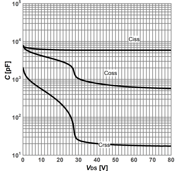
Diagram 12: Typ. capacitances
