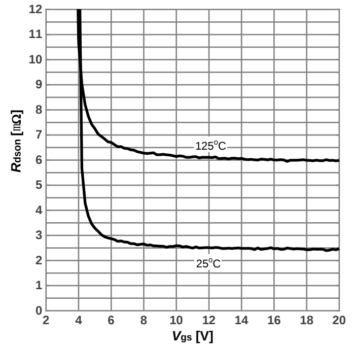
Diagram 11: On-state resistance vs. Vgs characteristics
