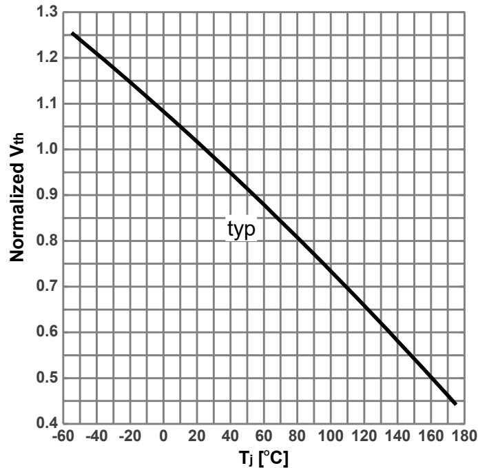
Diagram 7: Gate threshold voltage vs. Junction temperature
