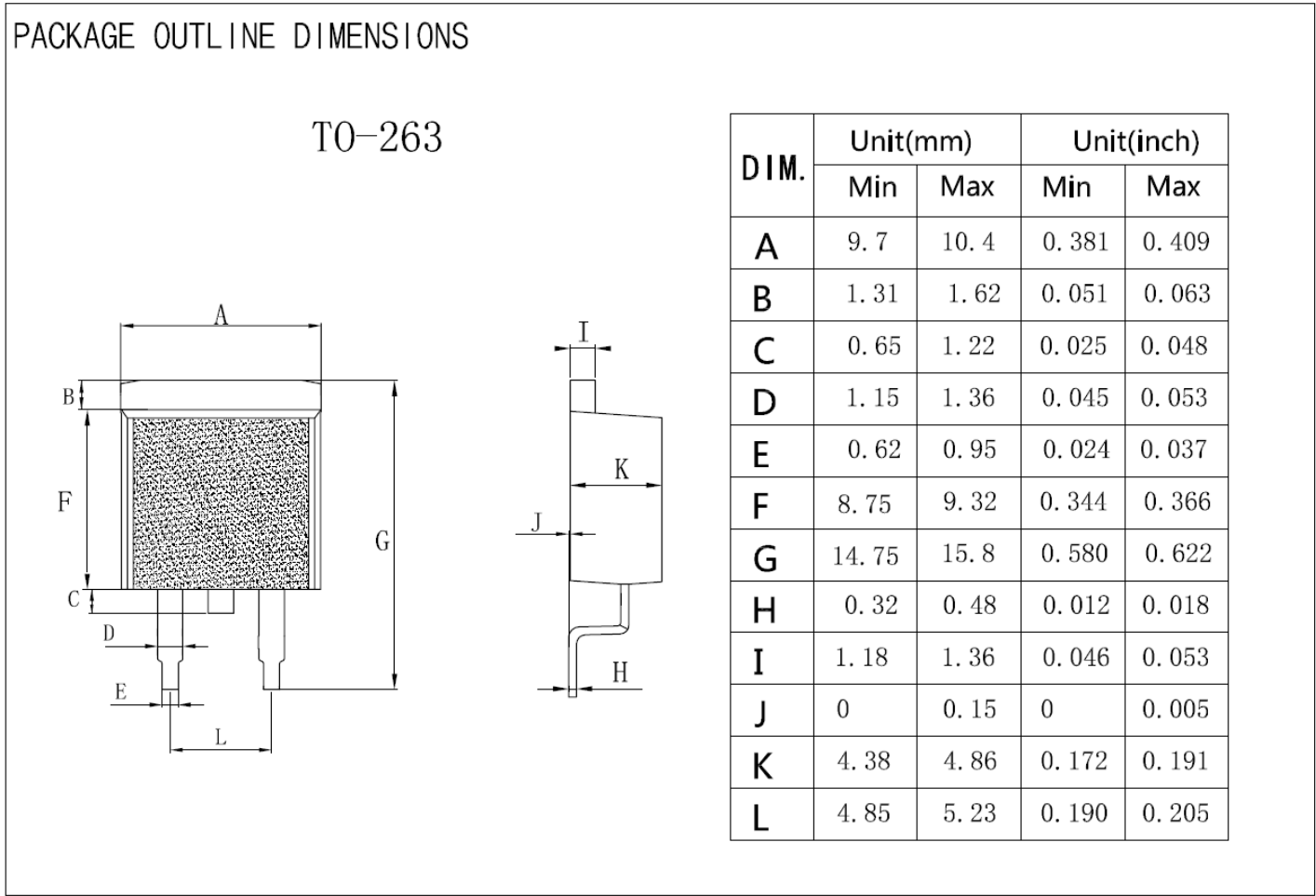
Figure 2 Outline TO-263 Dimensions in mm
