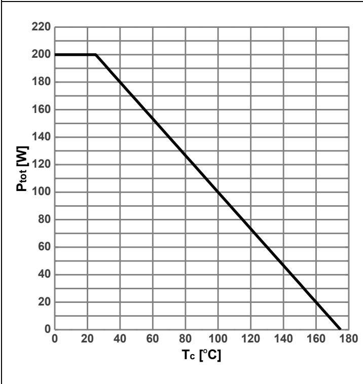
Diagram 1: Power Dissipation
