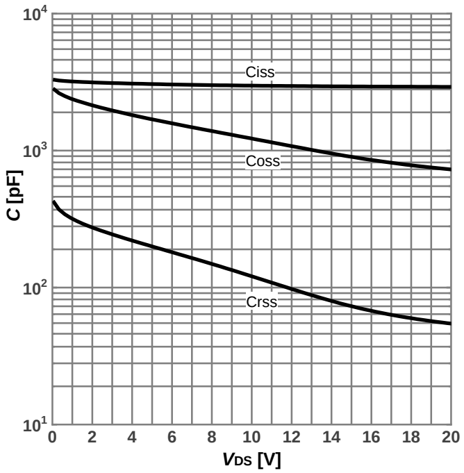
Diagram 12: Typ. Capacitances
