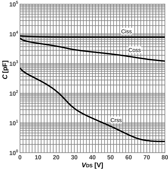
Diagram 12: Typ. capacitances
