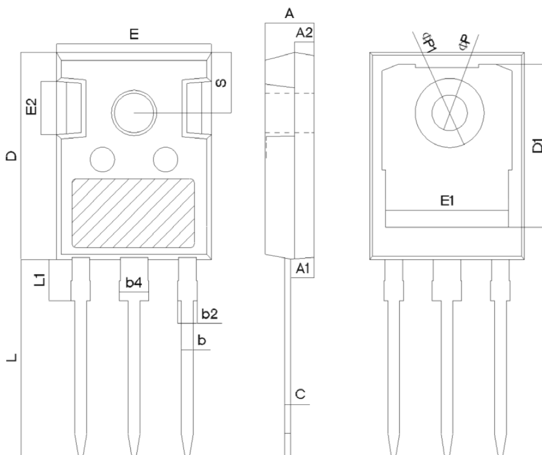
Figure 3 Outline TO-247 Dimensions in mm
