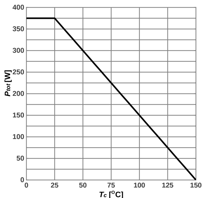
Diagram 1: Power dissipation
