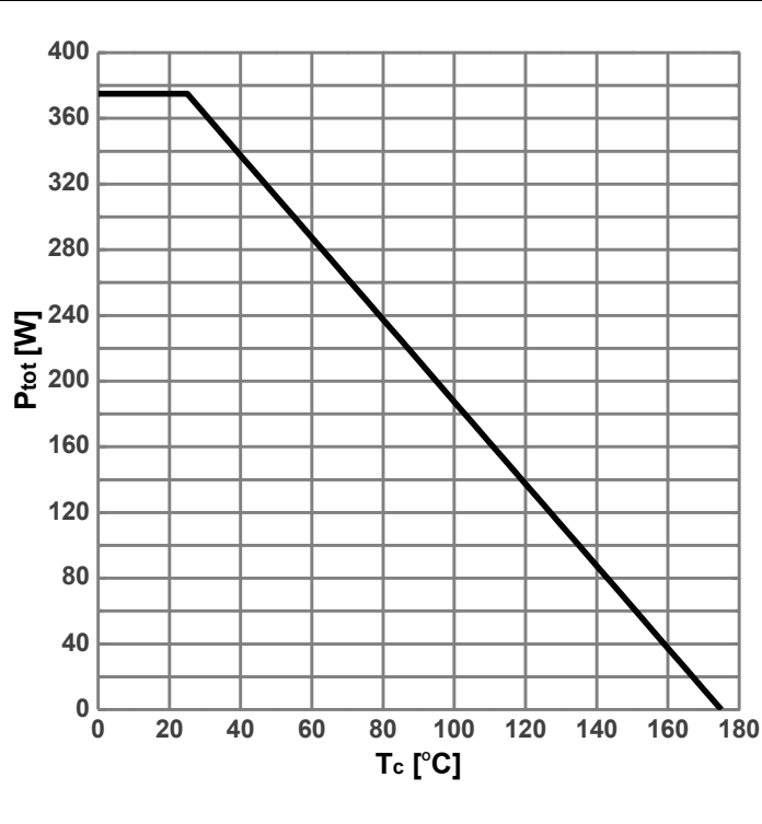
Diagram 1: Power dissipation
