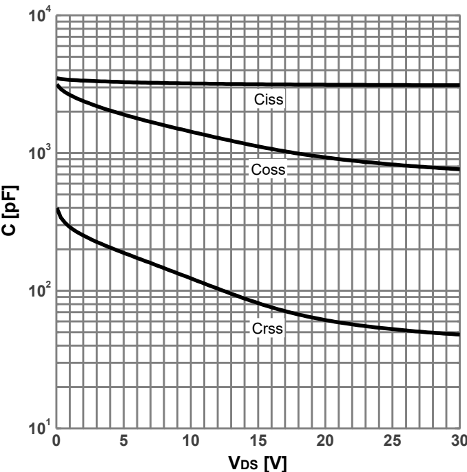
Diagram 12: Typ. capacitances
