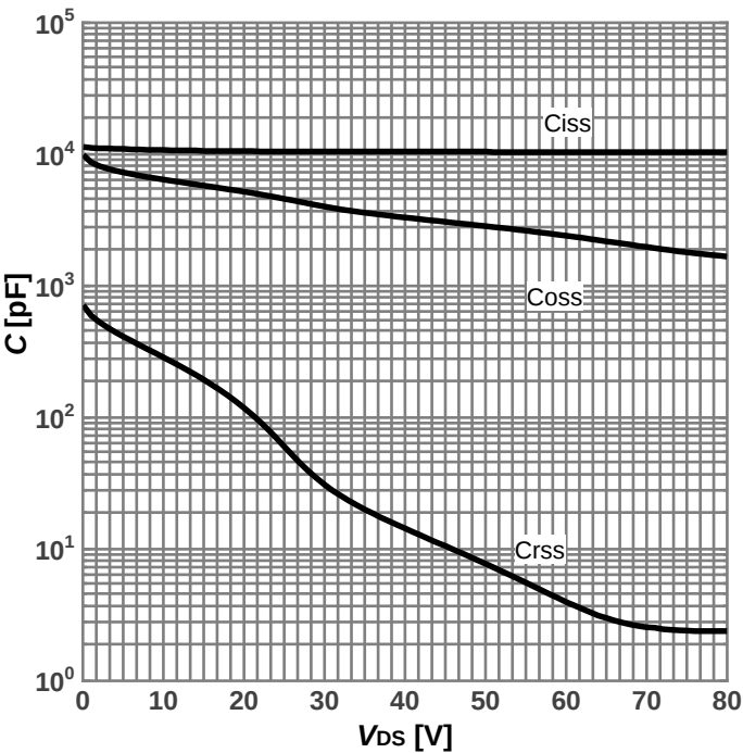
Diagram 12: Typ. capacitances
