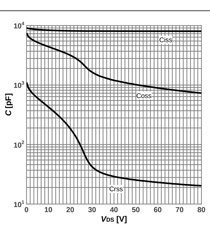
Diagram 12: Typ. Capacitances
