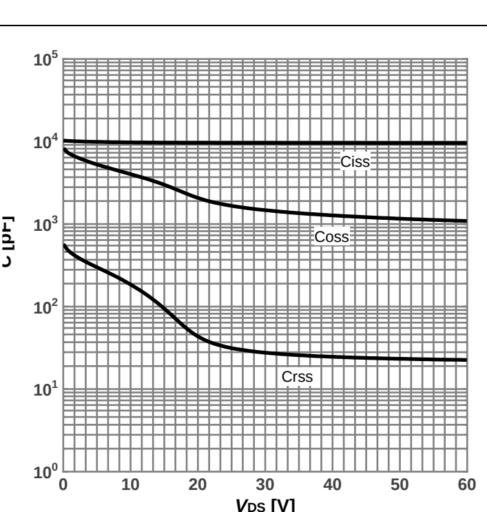
Diagram 12: Typ. capacitances
