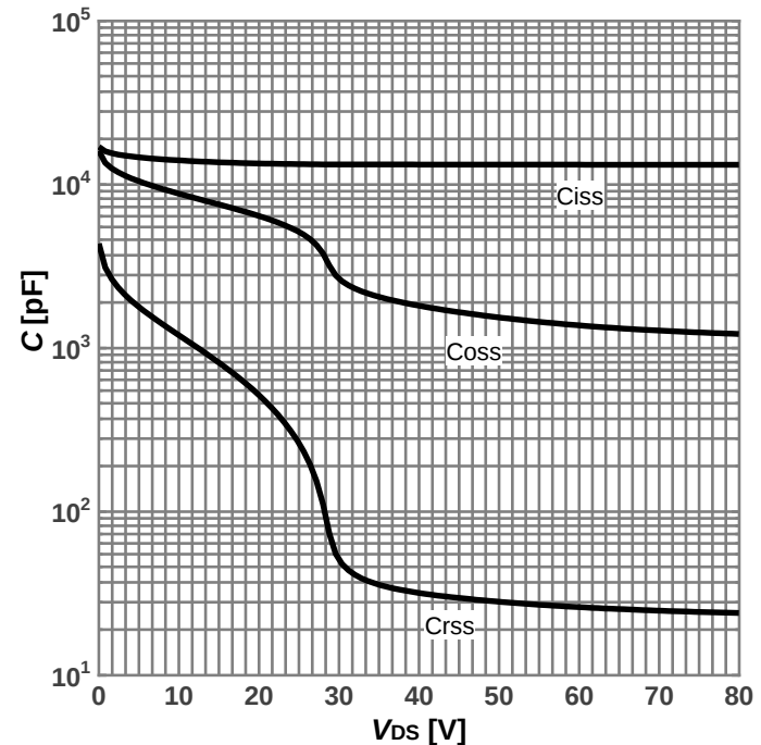
Diagram 12: Typ. capacitances
