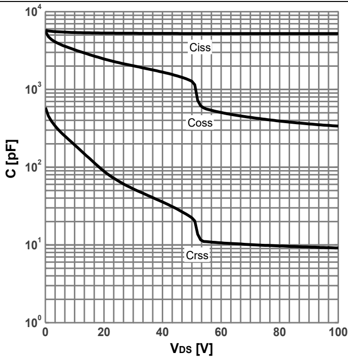
Diagram 13: Typ. capacitances
