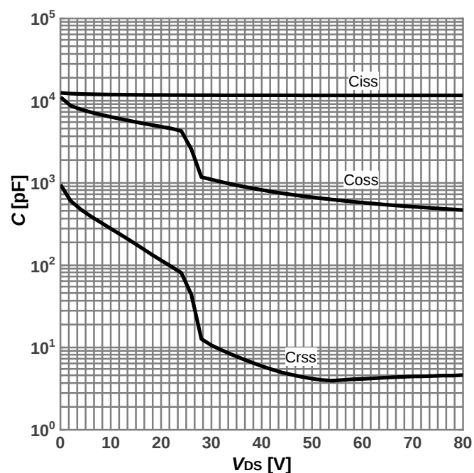
Diagram 12: Typ. capacitances
