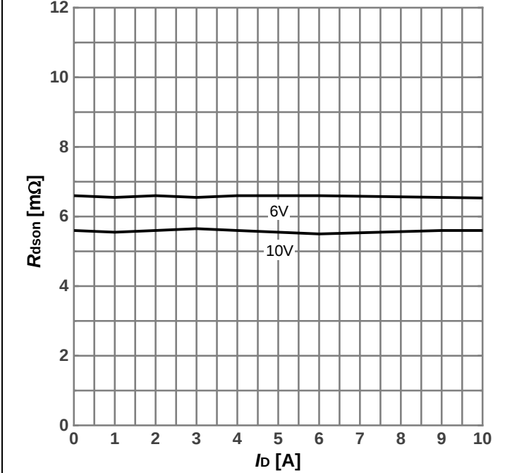
Diagram 7: On-state resistance vs. Drain current
