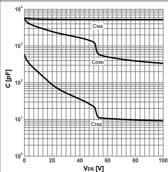
Diagram 12: Typ. capacitances
