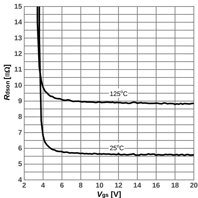
Diagram 10: On-state resistance vs. V_{GS} characteristics
