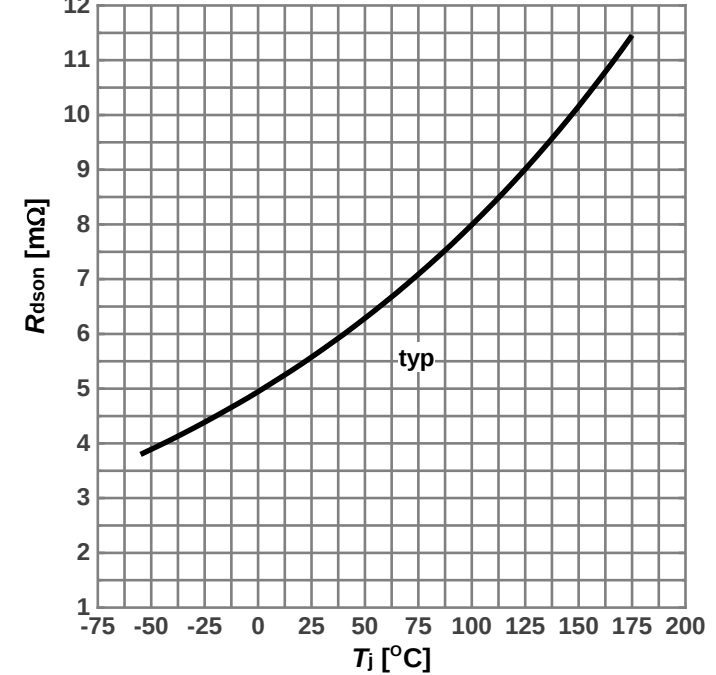
Diagram 8: On-state resistance vs. Junction temperature
