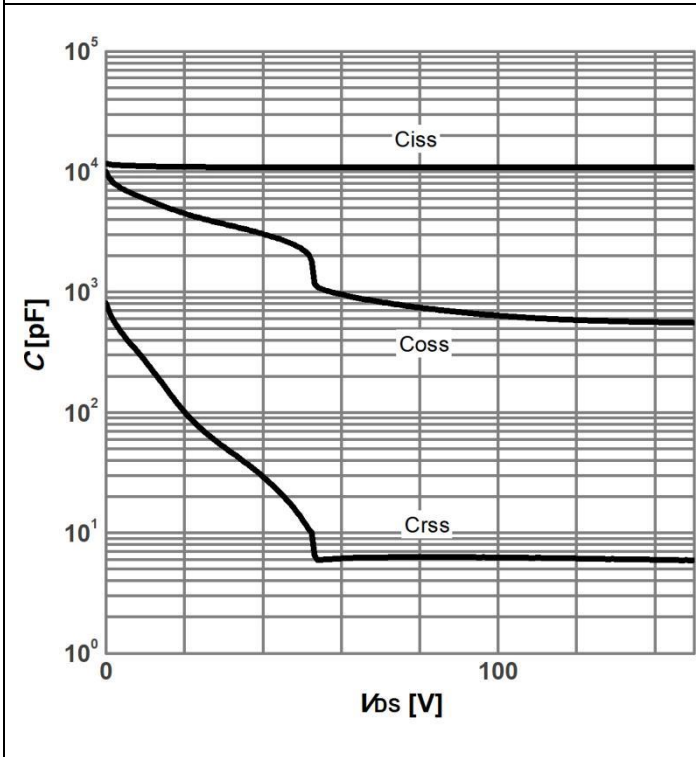
Diagram 13: Typ. capacitances
