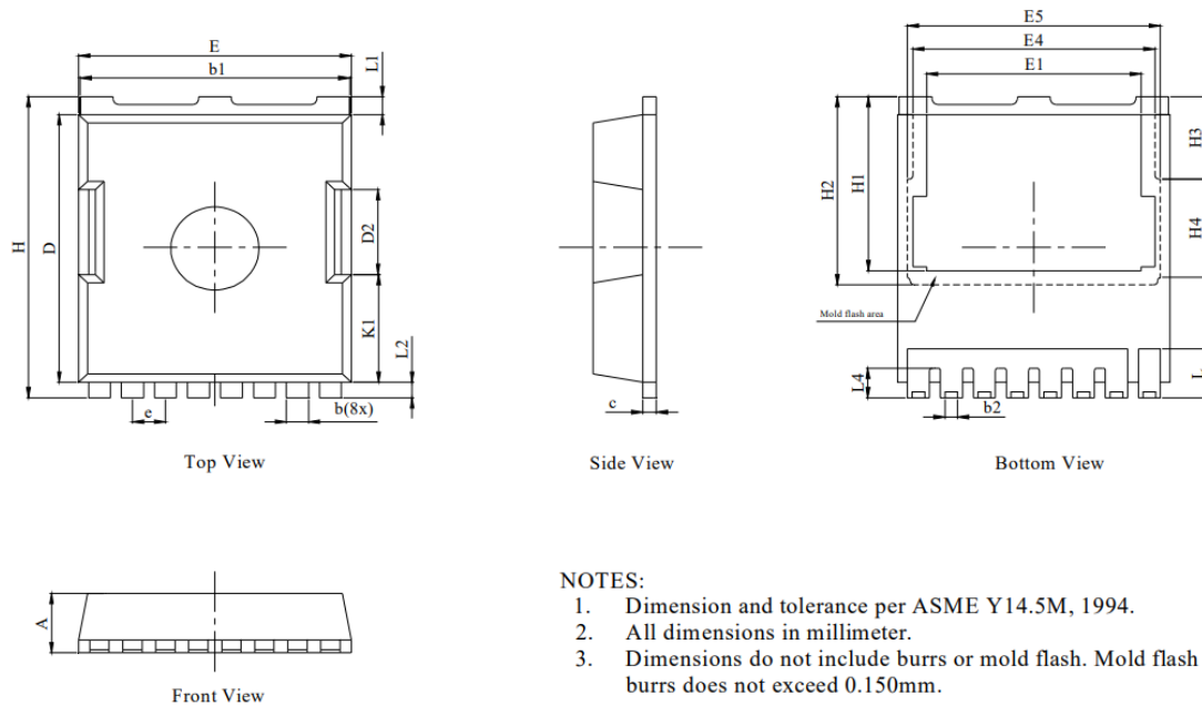
Figure 1 Outline TOLL Dimensions in mm
