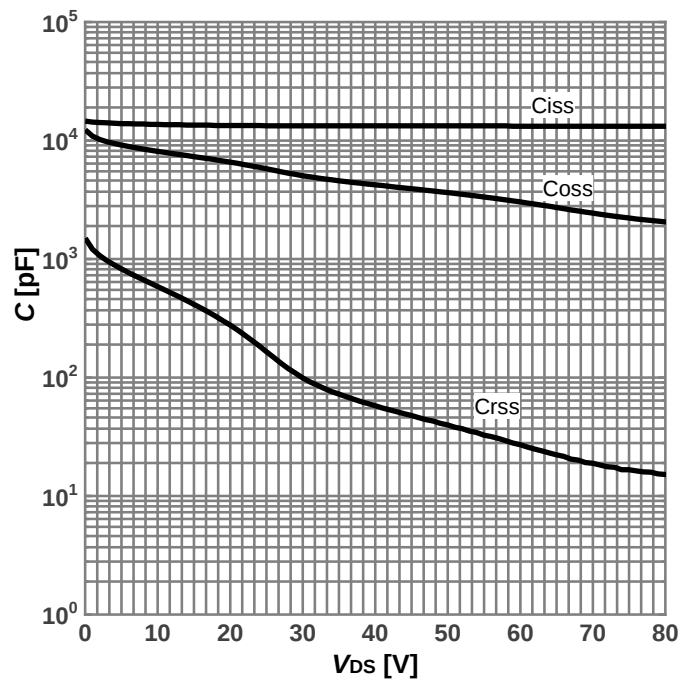
Diagram 12: Typ. capacitances
