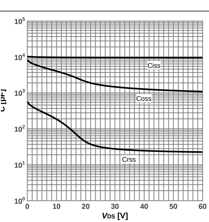
Diagram 12: Typ. capacitances
