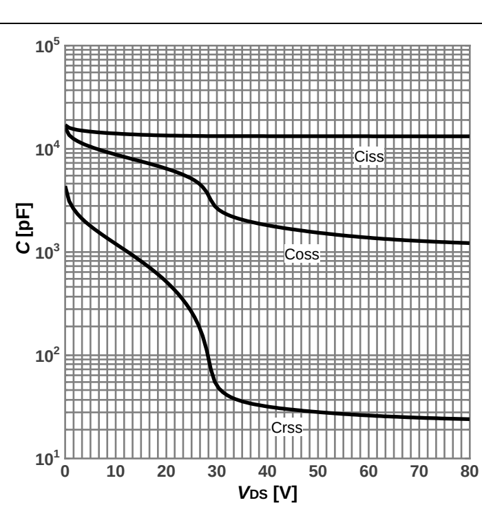
Diagram 12: Typ. capacitances
