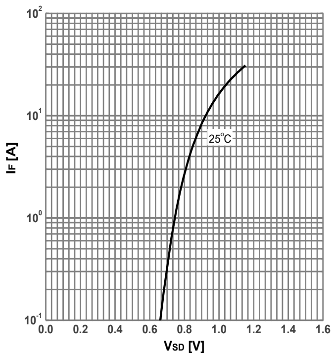
Diagram 10: Forward characteristics of reverse diode
