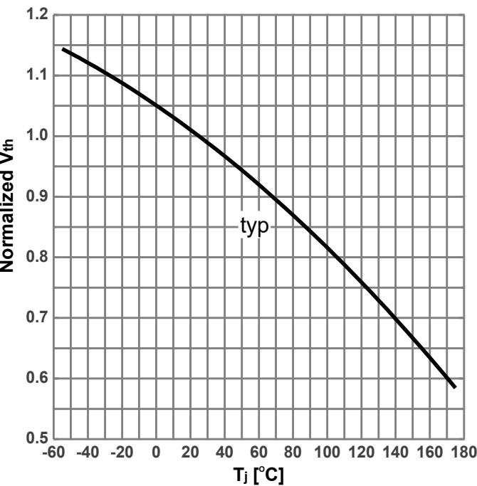
Diagram 7: Gate threshold voltage vs. Junction temperature
