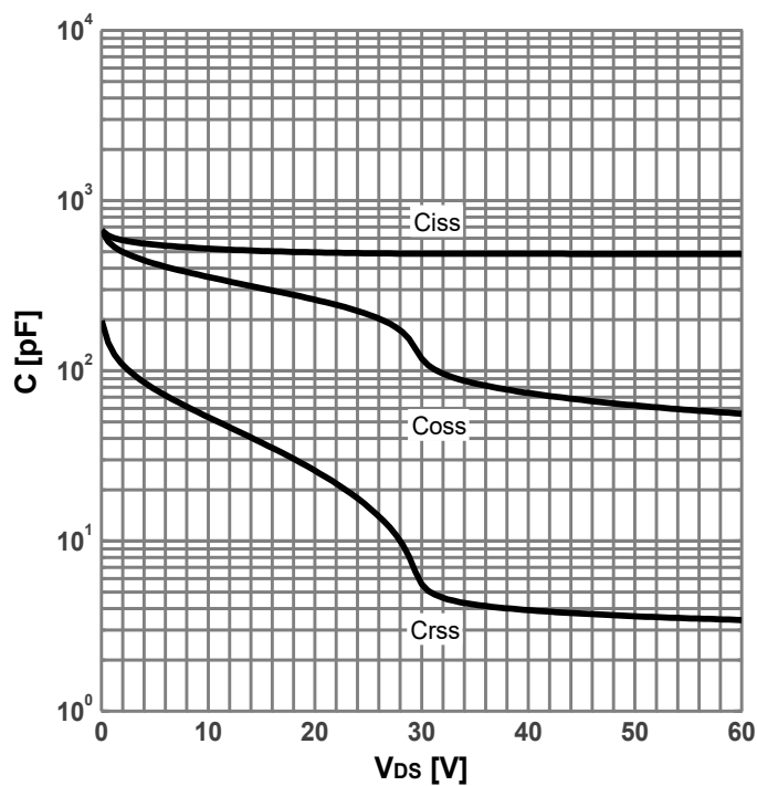
Diagram 12: Typ. capacitances
