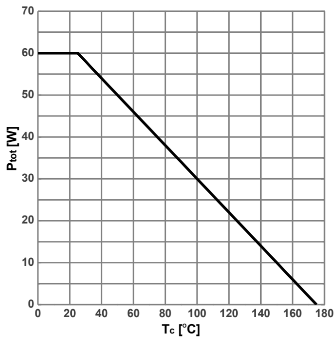
Diagram 1: Power dissipation
