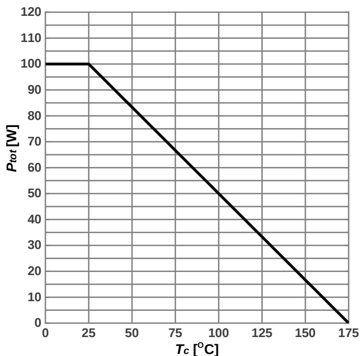
Diagram 1: Power dissipation
