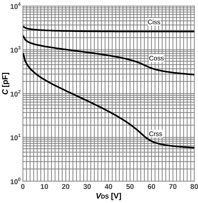
Diagram 12: Typ. capacitances
