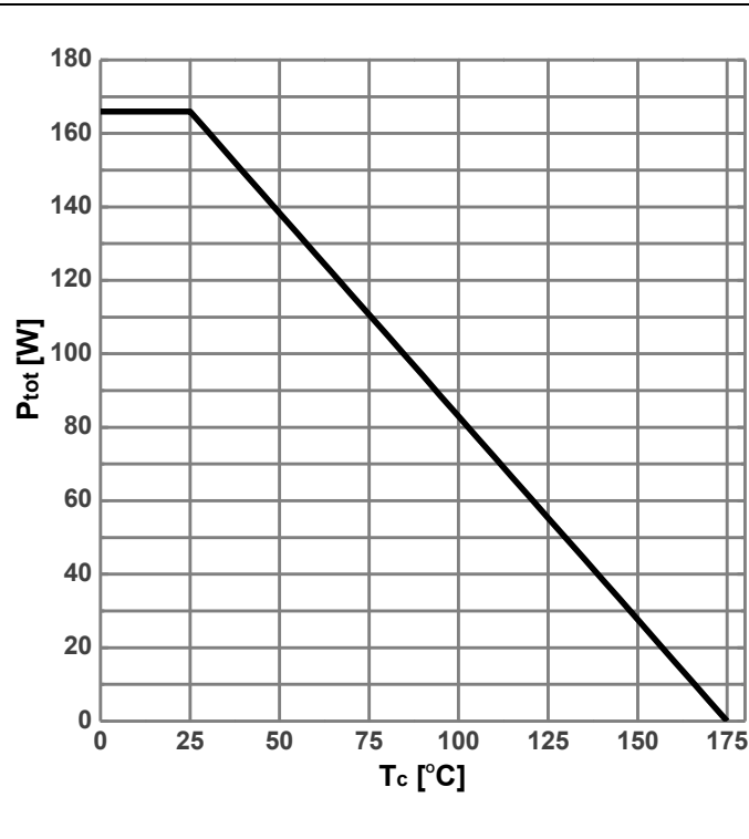
Diagram 1: Power Dissipation
