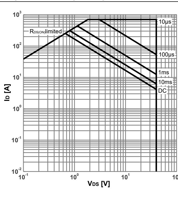
Diagram 3: Safe Operating Area
