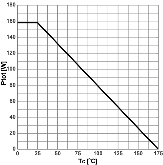
Diagram 1: Power dissipation
