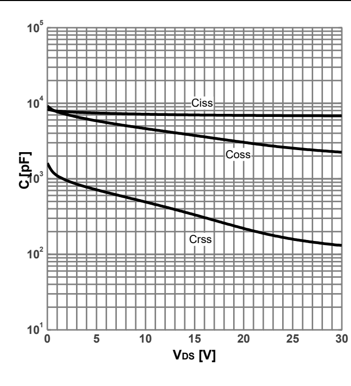
Diagram 12: Typ. capacitances
