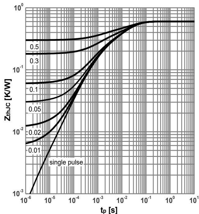
Diagram 2: Max. transient thermal impedance
