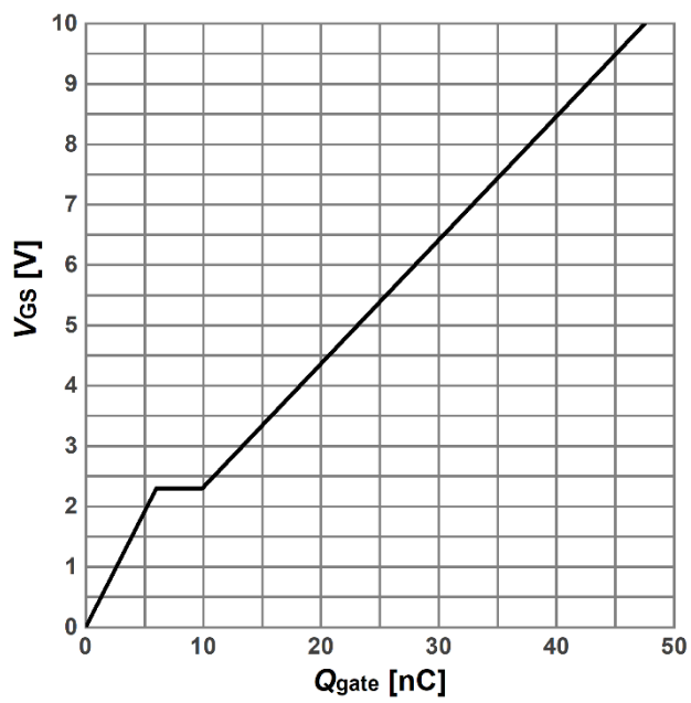
Diagram 13: Typ. gate charge
