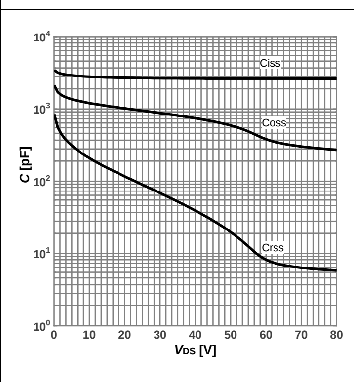
Diagram 12: Typ. capacitances
