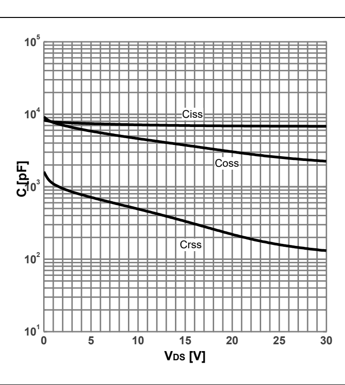
Diagram 12: Typ. capacitances
